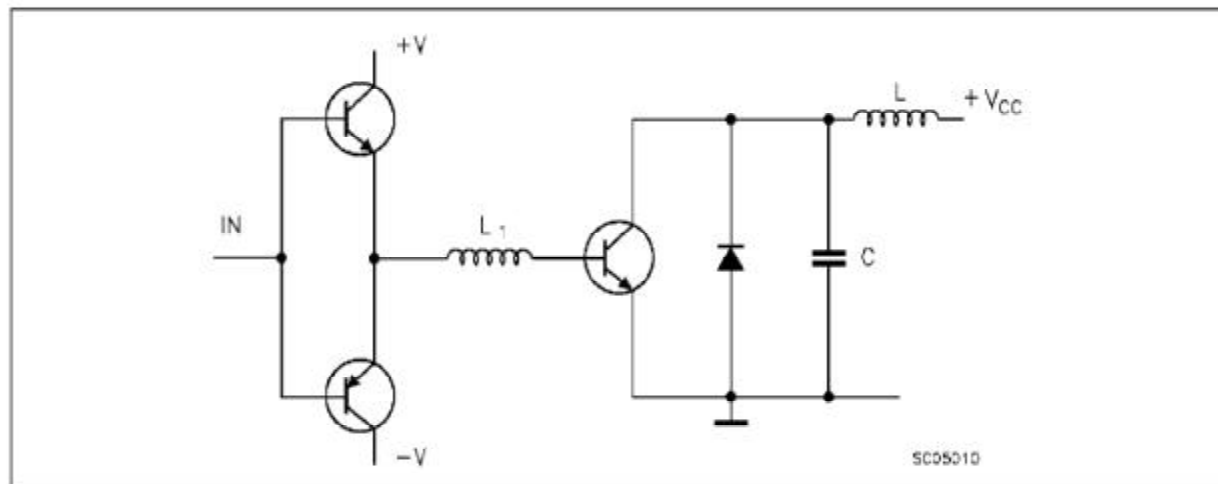
Figure 1: Inductive Load Switching Test Circuit.
