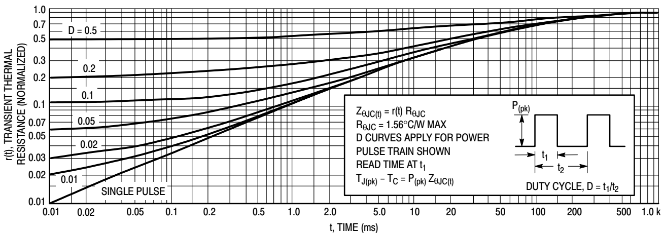
Figure 2. Thermal Response
