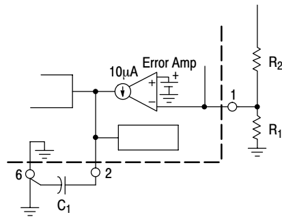
Figure 26. Error Amp Compensation
