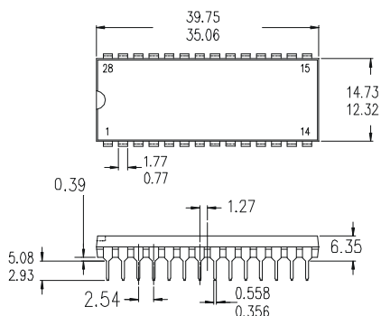
DIP-28
