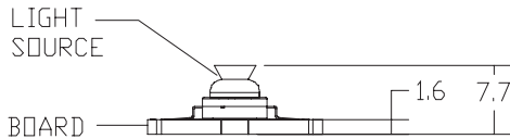
Side Emitting
